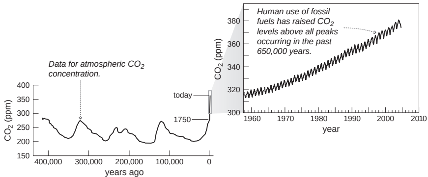
Figure 6.6. The carbon dioxide concentration in Earth's atmosphere over the past 400,000 years. Most of the data come from studies of air bubbles trapped in Antarctic ice (ice core samples); the data for the past half century (in the zoom-out) come from direct measurements made at Mauna Loa in Hawaii. (Illustration courtesy of Addison Wesley, an imprint of Pearson Education; data provided by the Carbon Dioxide Information Analysis Center)
