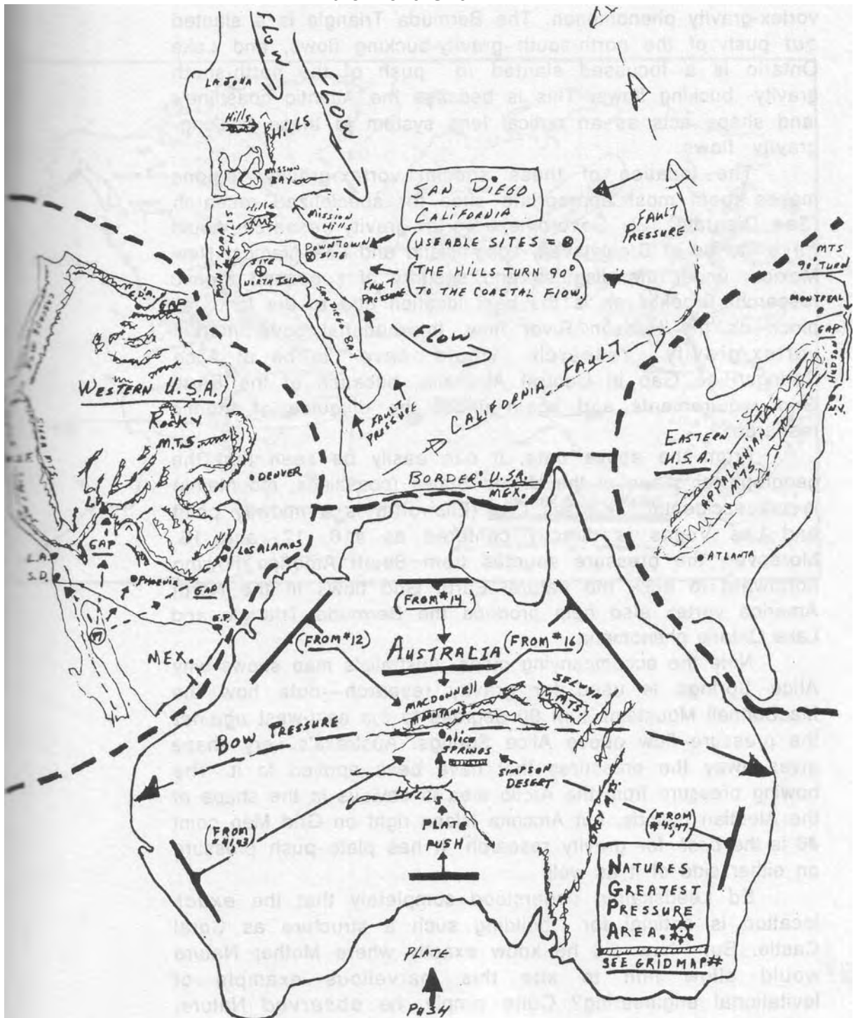
Worldwide Gravity Vortex Research Areas Plotted on the World Grid
