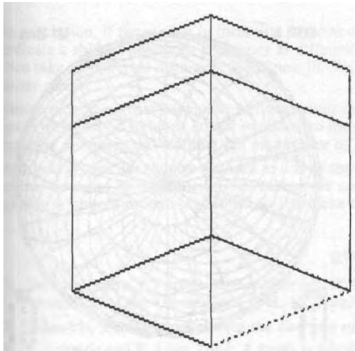
Figure 10. Right side view of the Rhombic Dodecahedron.
