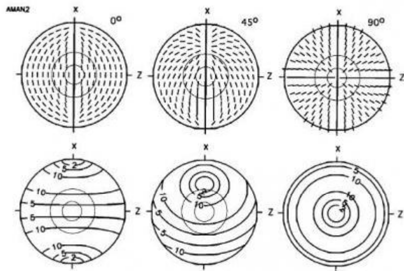
4.1. Examples of shear wave velocity patterns for horizontal and vertical shear waves.
