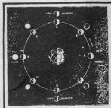
Phases of the Moon.
