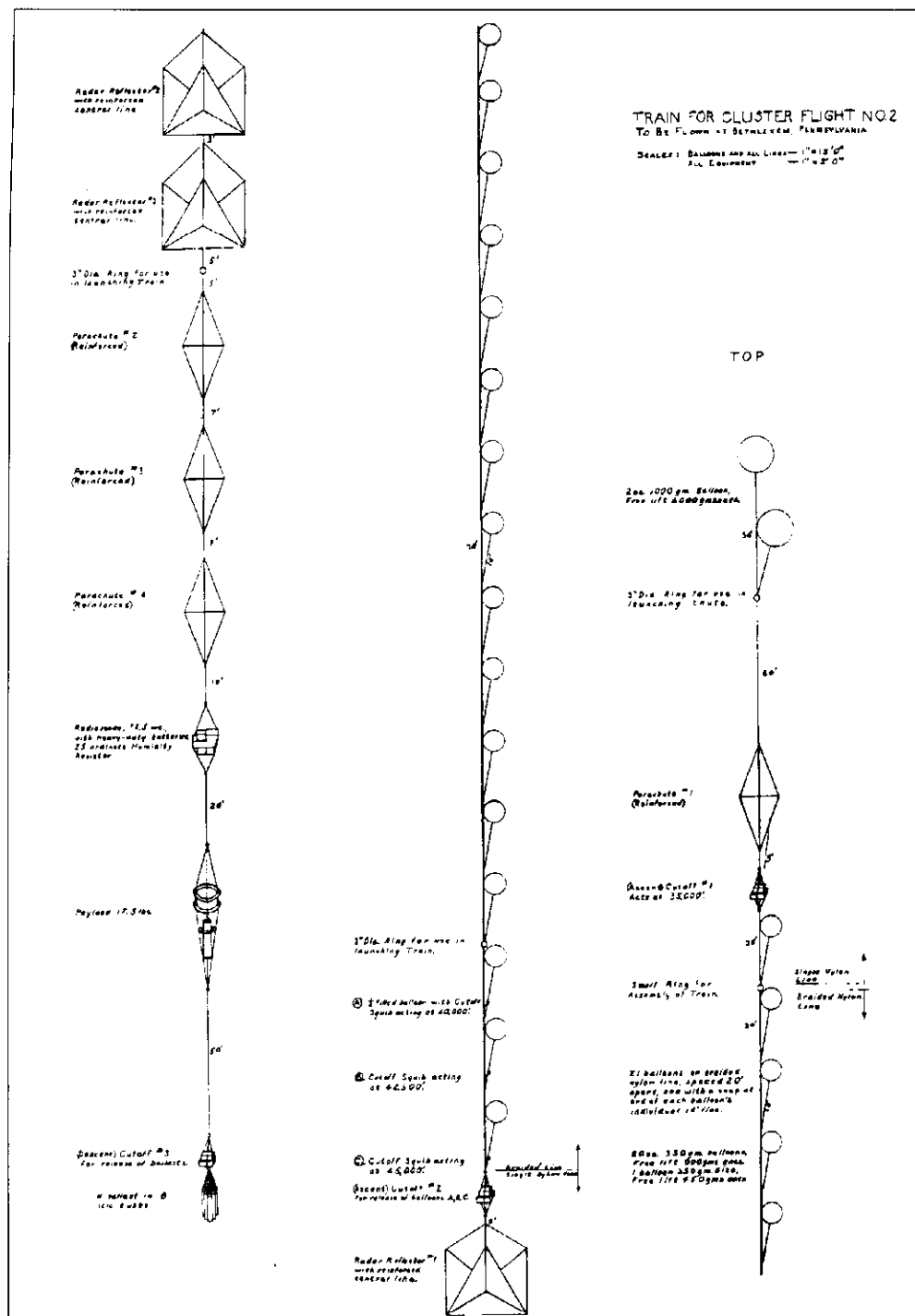
Fig. 3. An illustration of a Project MOGUL balloon train similar to one found on a ranch 75 miles northwest of Roswell, N.M. in June 1947, which contains all of the "strange" materials described as part of a "flying disc." Initial confusion at Roswell AAF and delayed identification of this equipment was the first in a series of unrelated events now known as the "Roswell Incident."
