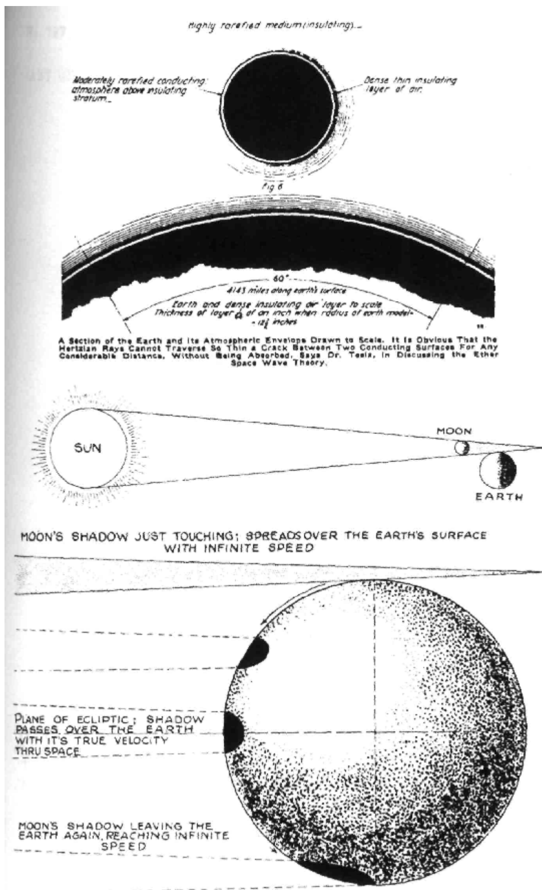
Above: Tesla's drawing of the earth and its atmospheric envelope drawn to scale from the February, 1919 issue of Electrical Experimenter , which discussed Tesla's "Ether Space Wave Theory." Below: Another drawing from 1929 demonstrating Tesla's Ether theory and how he theorized he would recover the energy from electromagnetic Hertz waves as oscillatory energy.
