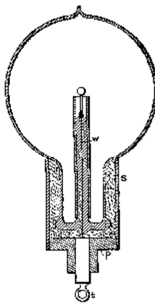
Fig. 19 – IMPROVED BULB WITH SOCKET AND SCREEN
