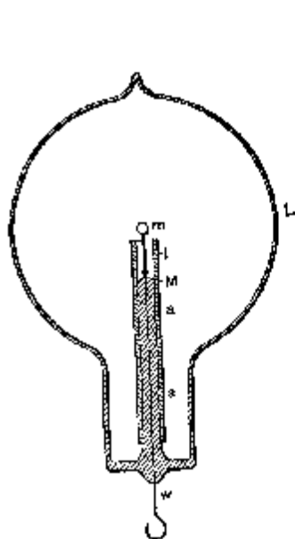
Fig. 18 – BULB WITH MICA TUBE AND ALUMINIUM SCREEN
