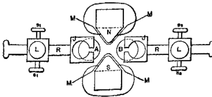
FIG. 4. — ARRANGEMENT OF IMPROVED DISCHARGER AND MAGNET.
